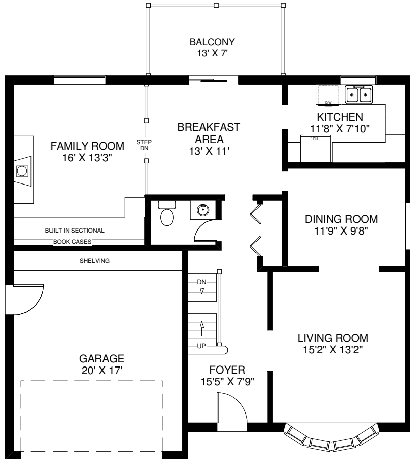
CEILING HT 8' MAIN FLOOR APPROXIMATELY 1,100 SQ FT
