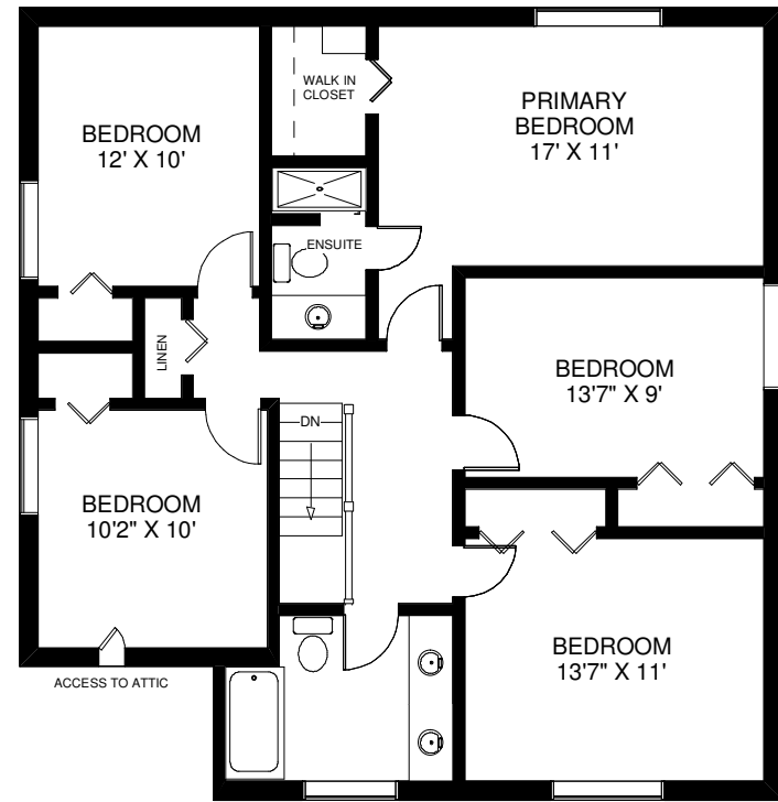
CEILING HT 8' SECOND FLOOR APPROXIMATELY 1,200 SQ FT
