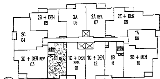
TYPICAL FLOOR (2nd-17th floor)
