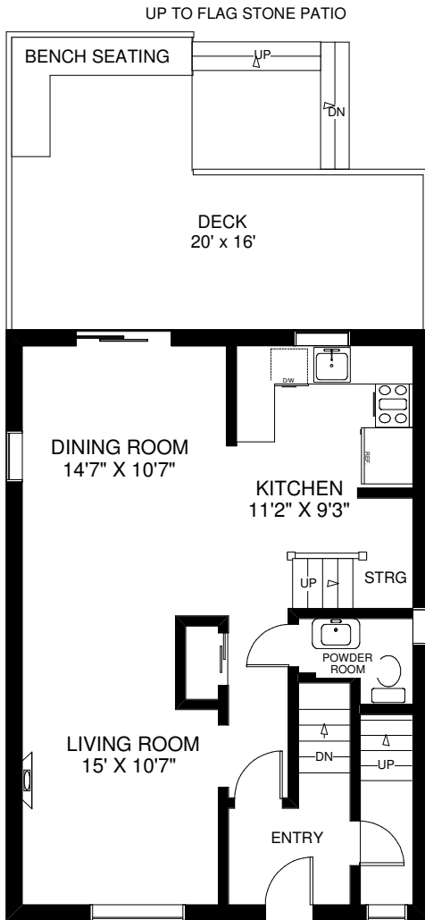
MAIN FLOOR APPROXIMATELY 685 SQ FT
