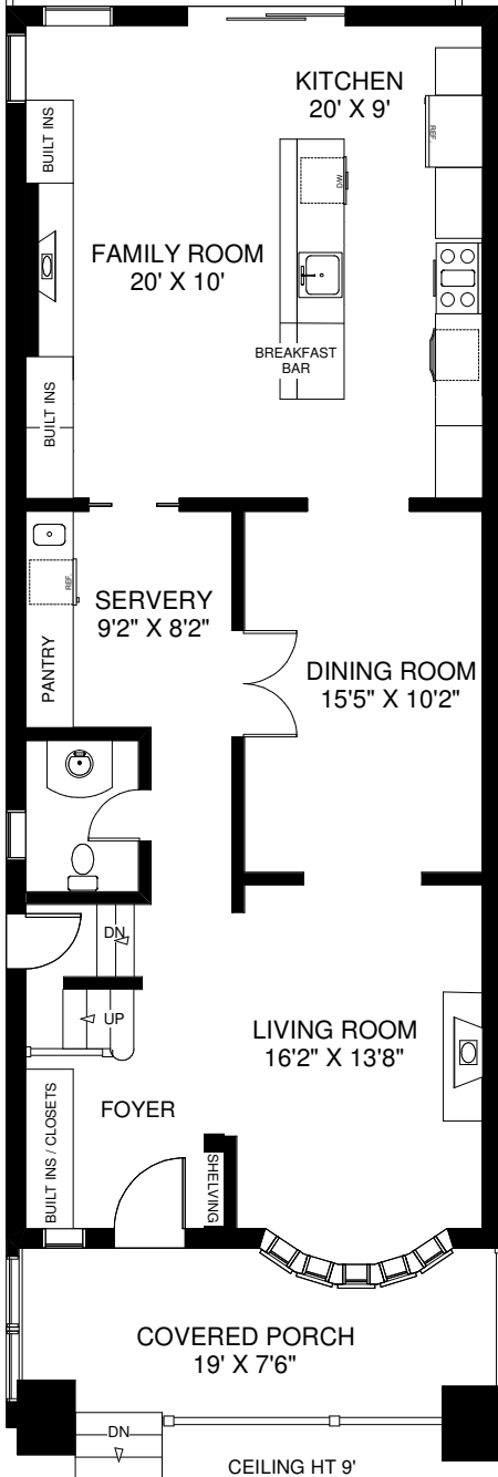
MAIN FLOOR APPROXIMATELY 1,115 SQ FT
