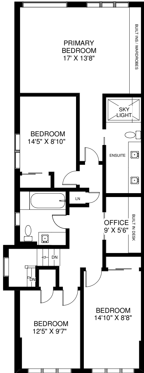
SECOND FLOOR APPROXIMATELY 1,200 SQ FT
